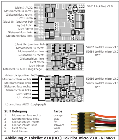
Abbildung 2: LokPilot V3.0 (DCC), LokPilot micro V3.0 - NEM651
