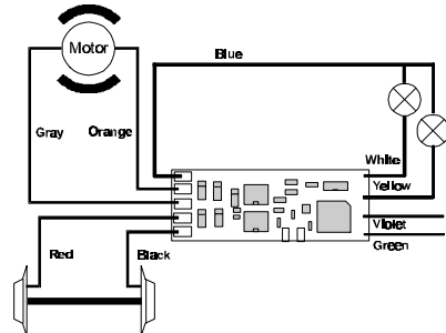
Figure 2: Wiring the LE080XS using a floating common.
