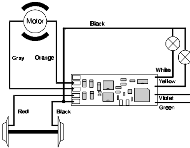
Figure 1: Wiring the LE080XS using track voltage common
