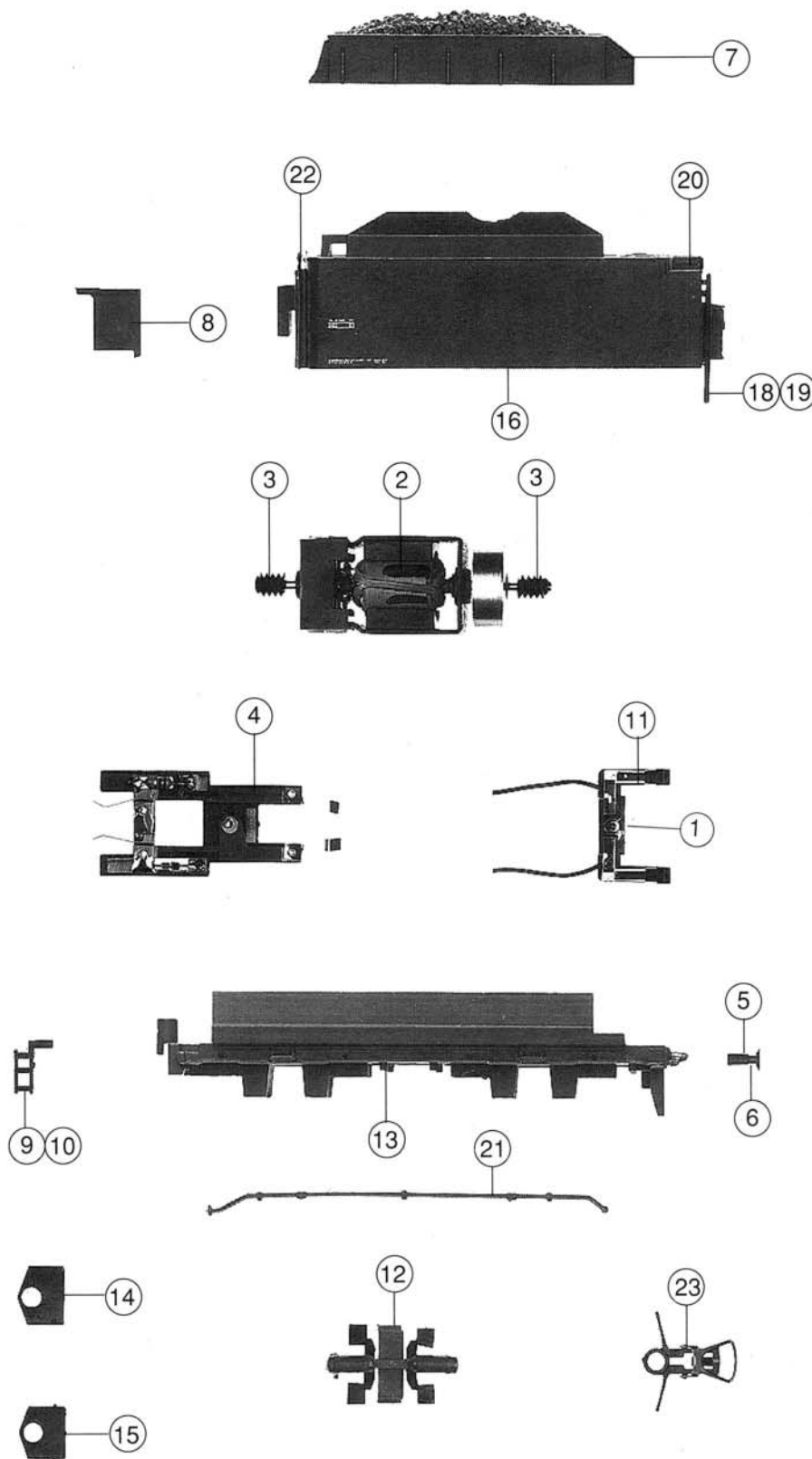
17 o. Abb. / no. ill. Tender komplett Tender assembly
