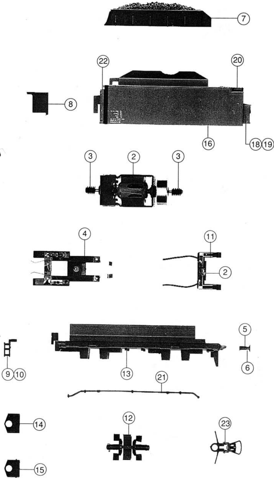
17 o. Abb. / no. ill. Tender komplett Tender assembly
